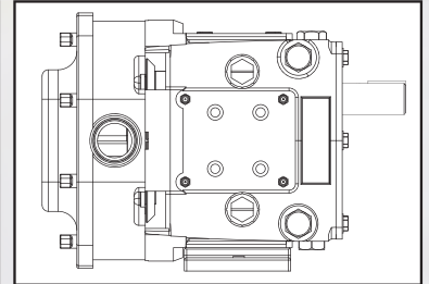
Upper Drive
